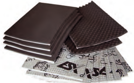
ESX QDK1 for damping two vehicle doors Thickness 1.8 mm, MLF 0.23
